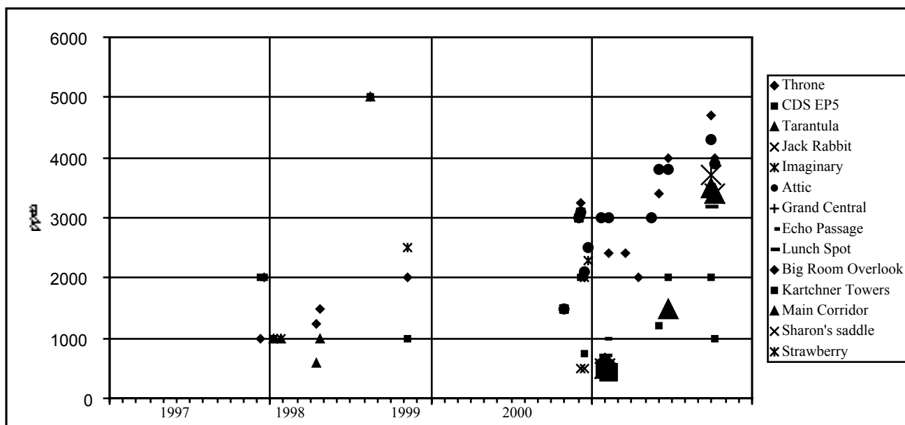
Fig. 3 - CO 2 concentrations in Kartchner Caverns from December 1997 to September 2000.
